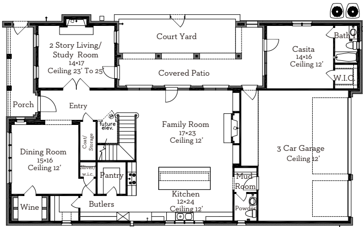
First Floor 2241 Sq.Ft
