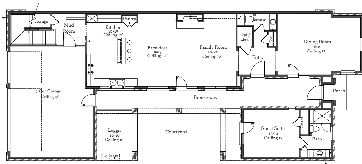
First Floor 1837 Sq.Ft
