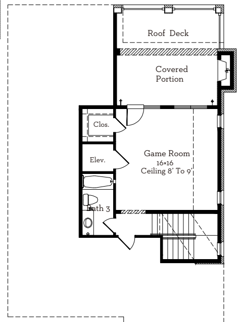
Third Floor 442 Sq.Ft
