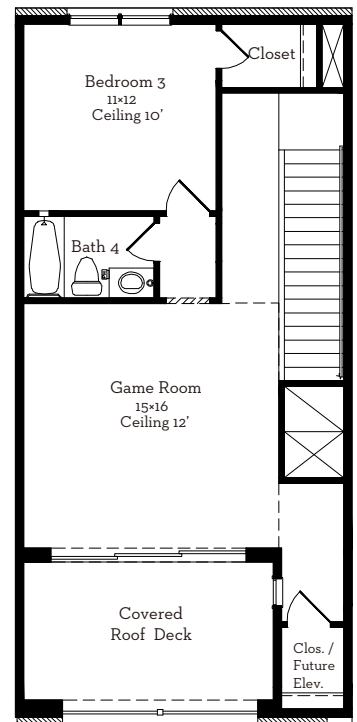
Fourth Floor 686 Sq.Ft
