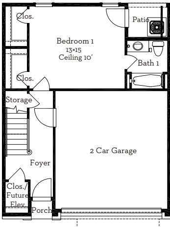
First Floor 510 Sq.Ft
