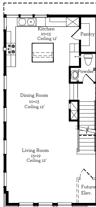
Second Floor 816 Sq.Ft
