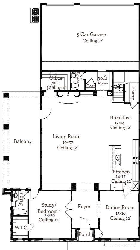
First Floor 2098 Sq.Ft
