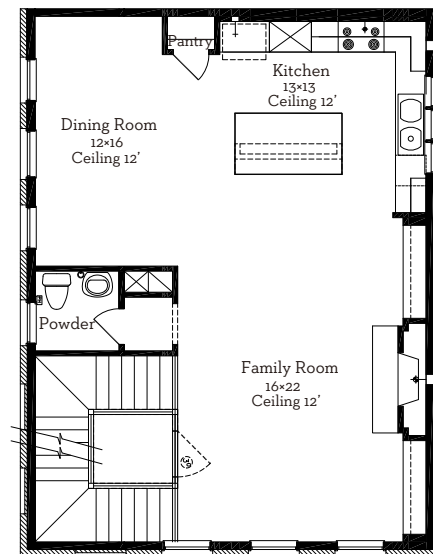
Second Floor 957 Sq.Ft
