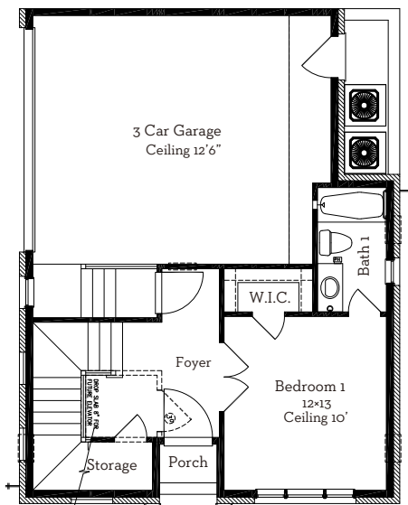
First Floor 460 Sq.Ft
