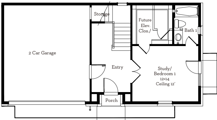
First Floor 502 Sq.Ft
