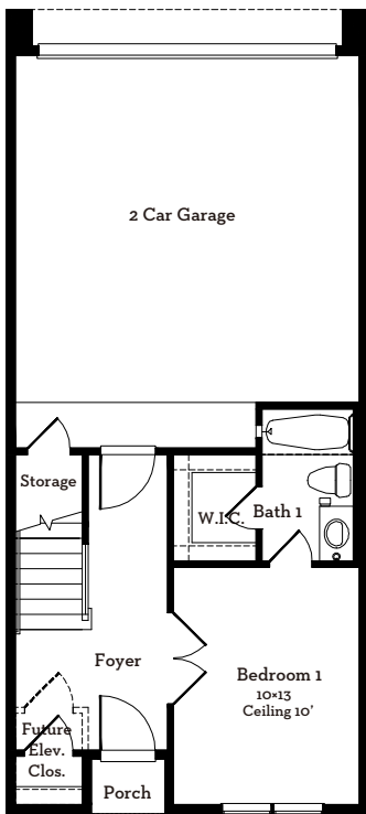
First Floor 403 Sq.Ft
