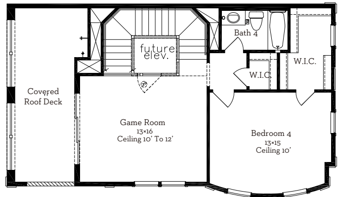
Fourth Floor 656 Sq.Ft
