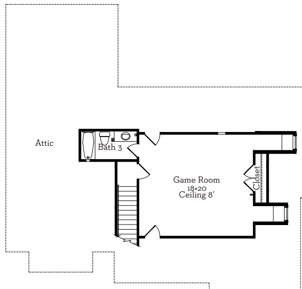
Third Floor 536 Sq.Ft
